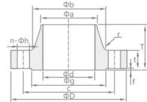
WN of nominal size 10A to 400A
